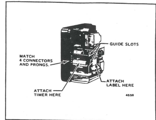
Fig. 1—Location of ST71A Timer and Label for R4795 Primary Control.
