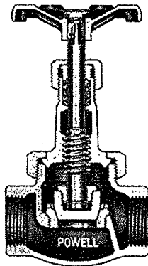
Fig. 2608 Class 200 Globe, Threaded Sizes, 1/4" through 3"
